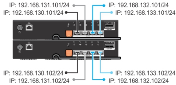
Figure 2. Four Hosts Connected to Two Controllers
