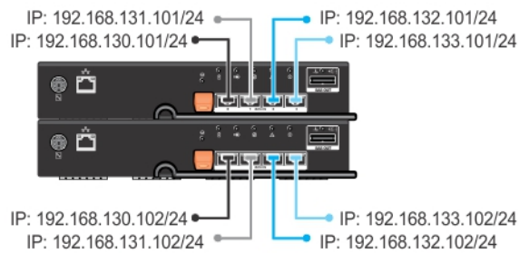
Figure 3. Four Cluster Nodes Connected to Two Controllers
