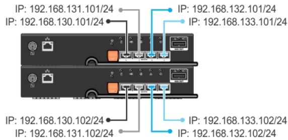
Figure 1. Eight Hosts With a Single Data Path
