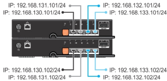
Figure 5. Initiator Configuration
